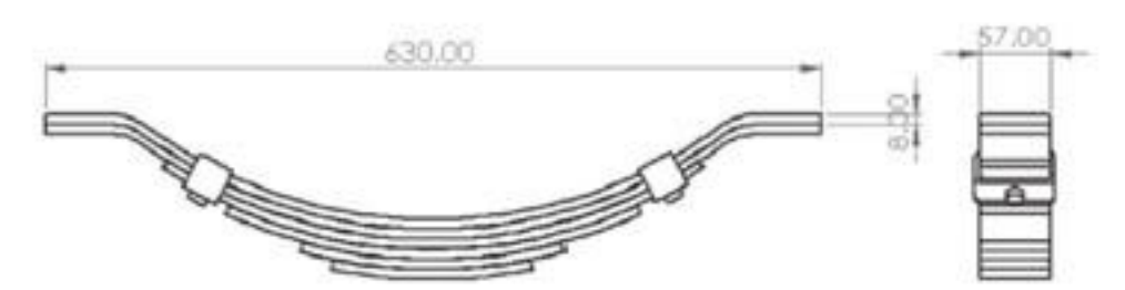
Standart Makas
